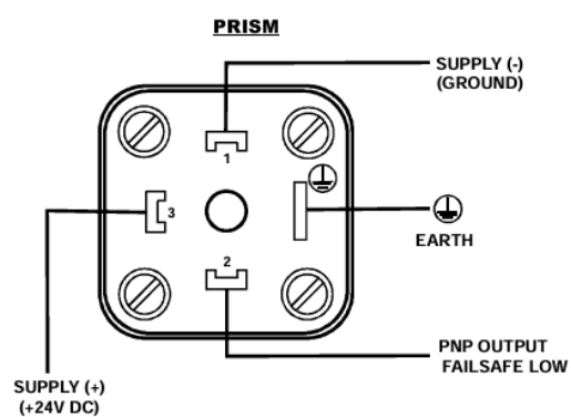
ELECTRICAL CONNECTION- 24V-DC DIN CONNECTOR
