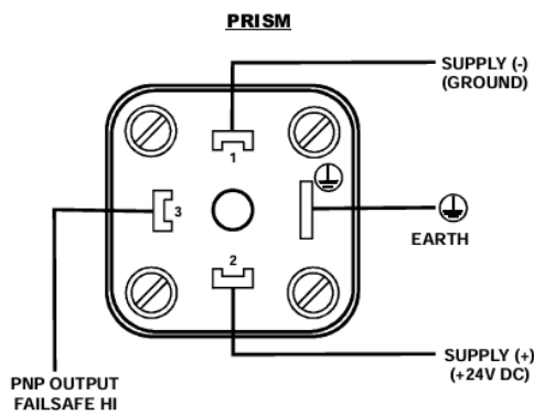
ELECTRICAL CONNECTION- 24V-DC DIN CONNECTOR
